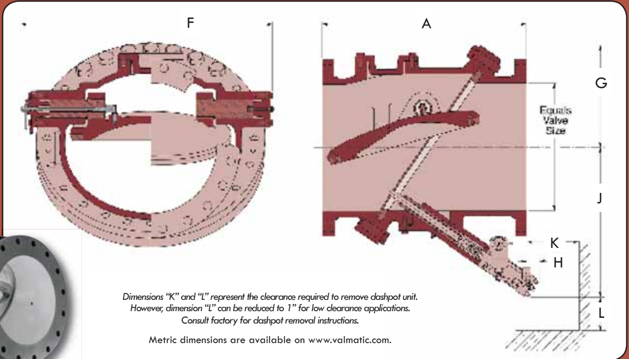
Integral disc ring and bushings on sizes 10" and smaller
